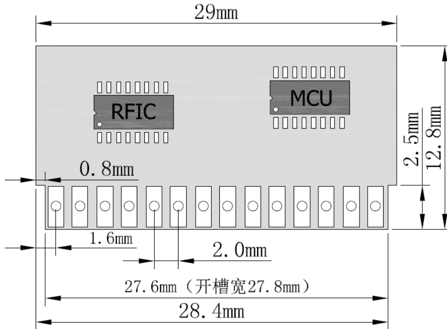
Figure 4: DL-RX06C-LO6 Dimensions
