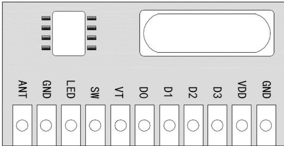
Figure4 DL-RXC6A Module interface definition diagram
