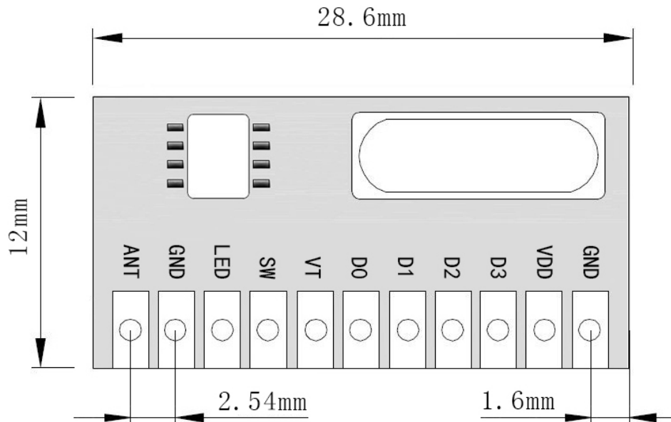
Figure6: DL-RXC6A Dimensions
