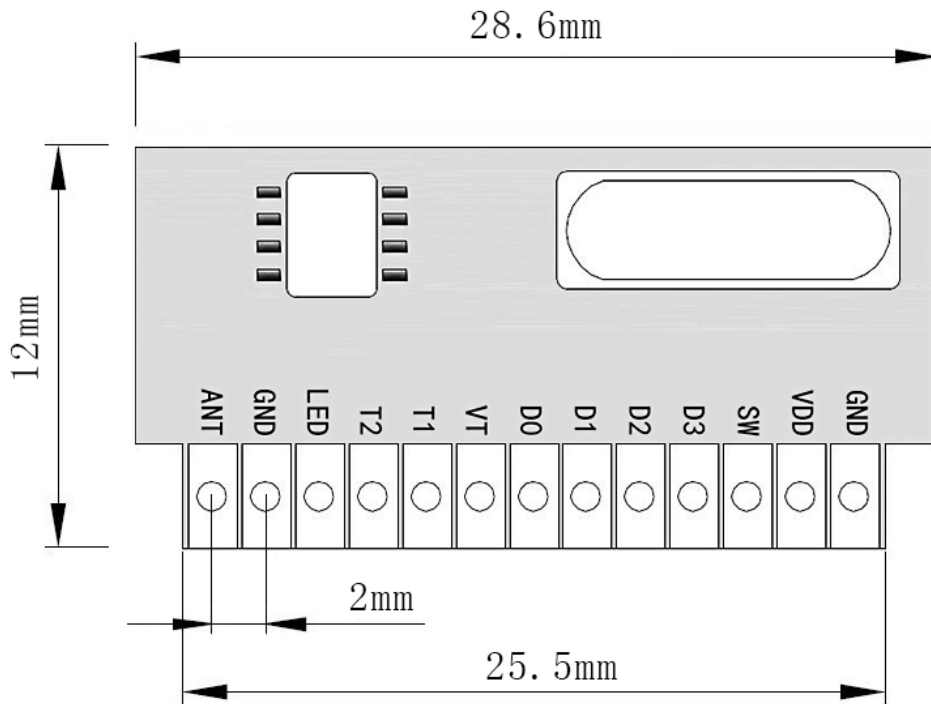
Figure 7: DL-RXC6B Dimensions ( Recommended slot length 26mm, slot width 1.1mm )
