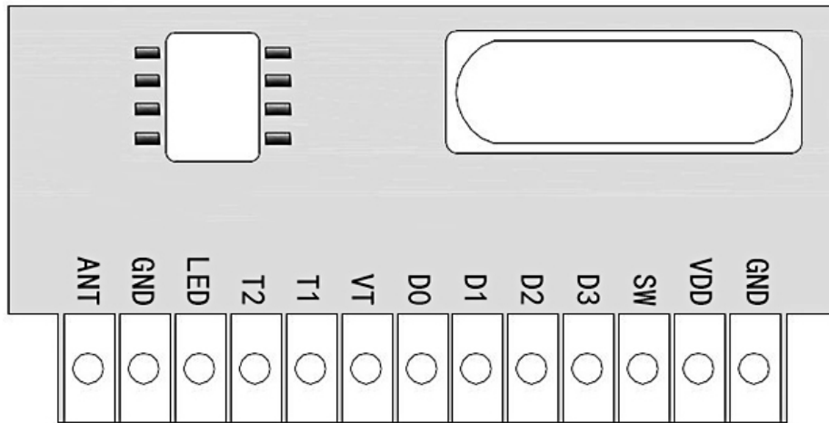
Figure 5 DL-RXC6B Module interface definition diagram
