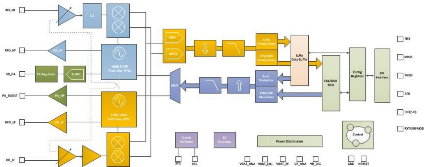
Figure 3. DL-RFM95/96/98 Block Schematic Diagram
