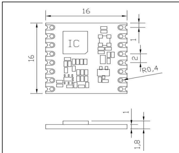
Figure 57:Package Outline Drawing
