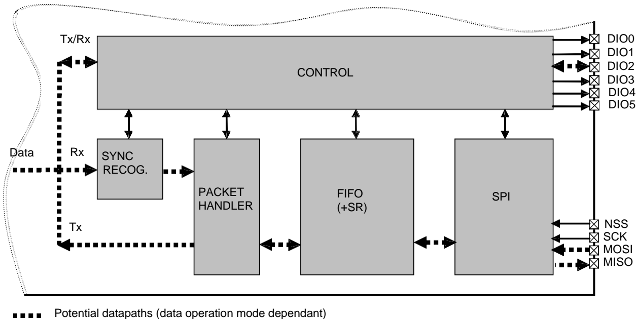
Figure 25. DL-RFM95/96/98 Data Processing Conceptual View
