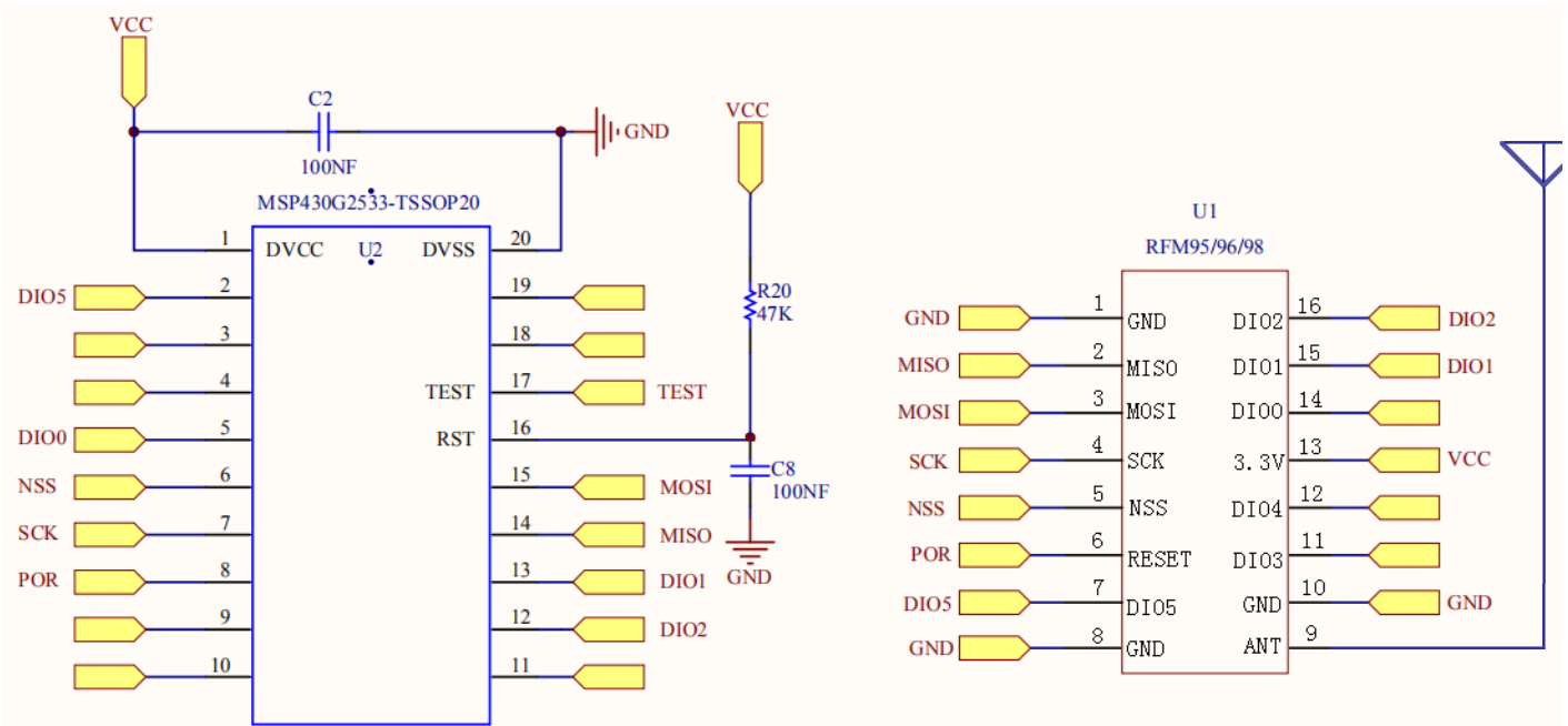
Figure 56:Reference Schematic
